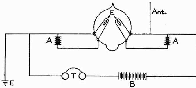
FIG. 2. Plan for an early carbon filament detector (1904). A = "A" batteries. B = "B" battery. E = earth. T = telephone.
